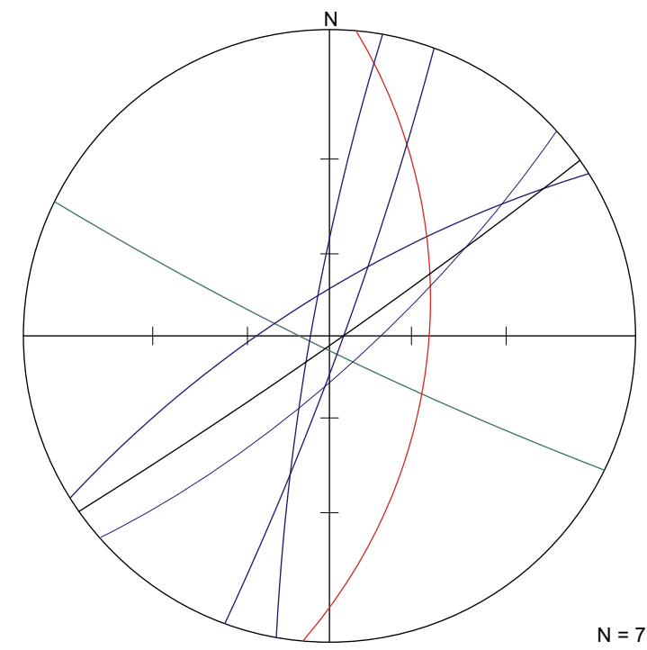
Traces of faults (Equal Angle, Wulff net)
