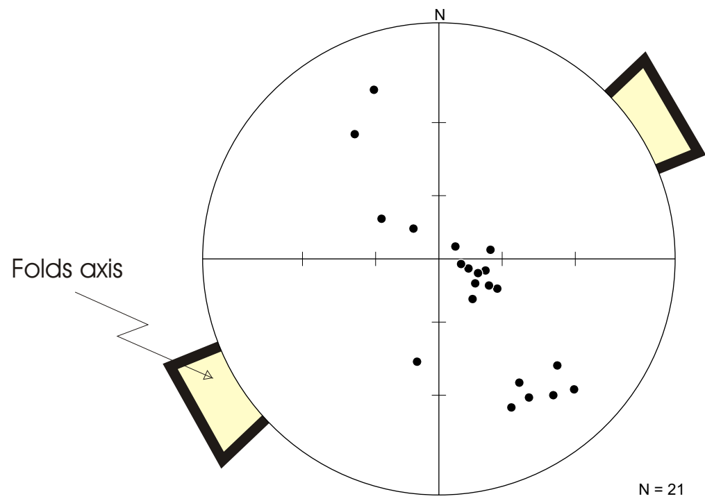
Poles of S0 (Equal Angle, Wulff net)
